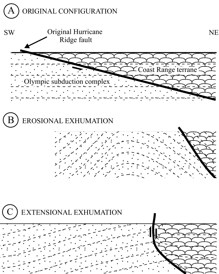
Figure 14. Schematic cross sections illustrating the pattern of exhumation that would result from tectonic and erosional exhumation. (A) The original configuration of the margin was formed by accretion of the Olympic subduction complex beneath the truncated base of the Coast Range terrane. The horizontal dashed lines schematically illustrate depth contours associated with this initial configuration. (B) Erosional exhumation would be distinguished by an exhumation pattern centered over the area of greatest tectonic uplift. In this case, the Hurricane Ridge fault is passively tilted into its present steep orientation. (C) Extensional exhumation caused by normal faulting on the Hurricane Ridge fault would result in an asymmetric pattern with the deepest exposures located directly west of the fault.
