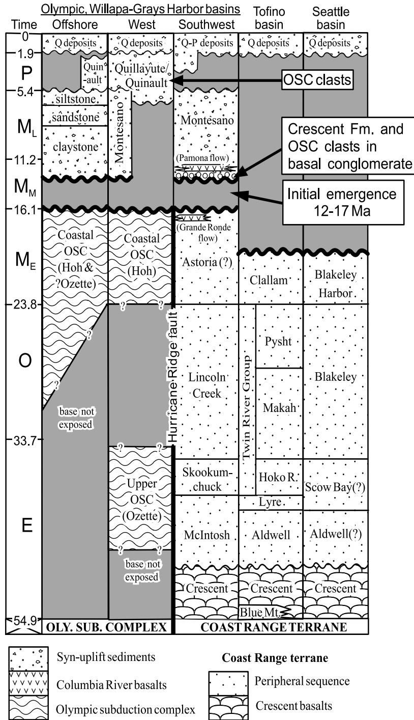
Figure 3. Summary of stratigraphic evidence for emergence and erosion of the Olympic Mountains starting in middle Miocene time. The locations of the cited basins are shown in Figure 2. Data sources: Offshore and West columns: Rau (1975, 1979), Snively et al. (1986, 1993), Palmer and Lingley (1989); Southwest column: Armentrout et al. (1983, 1988), Walsh et al. (1987); Tofino column: Snively et al. (1980), Garver and Brandon (1994); Seattle column: Armentrout et al. (1983, 1988), Squires et al. (1992), Johnson et al. (1994). OSC—Olympic subduction complex; E—Eocene; O—Oligocene; M—Miocene (E—early, M—middle, L—late); P—Paleocene; Fm.—formation; Q—Quaternary.
